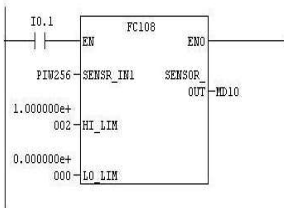
Fig. 7: FC 108 Block
