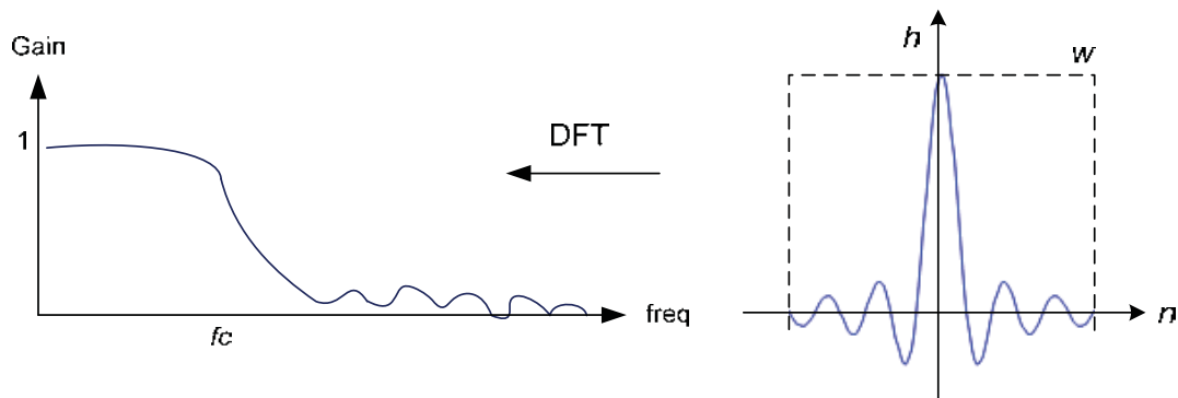
Figure 4.20: Truncated impulse response for LPF and Gibbs phenomenon.
