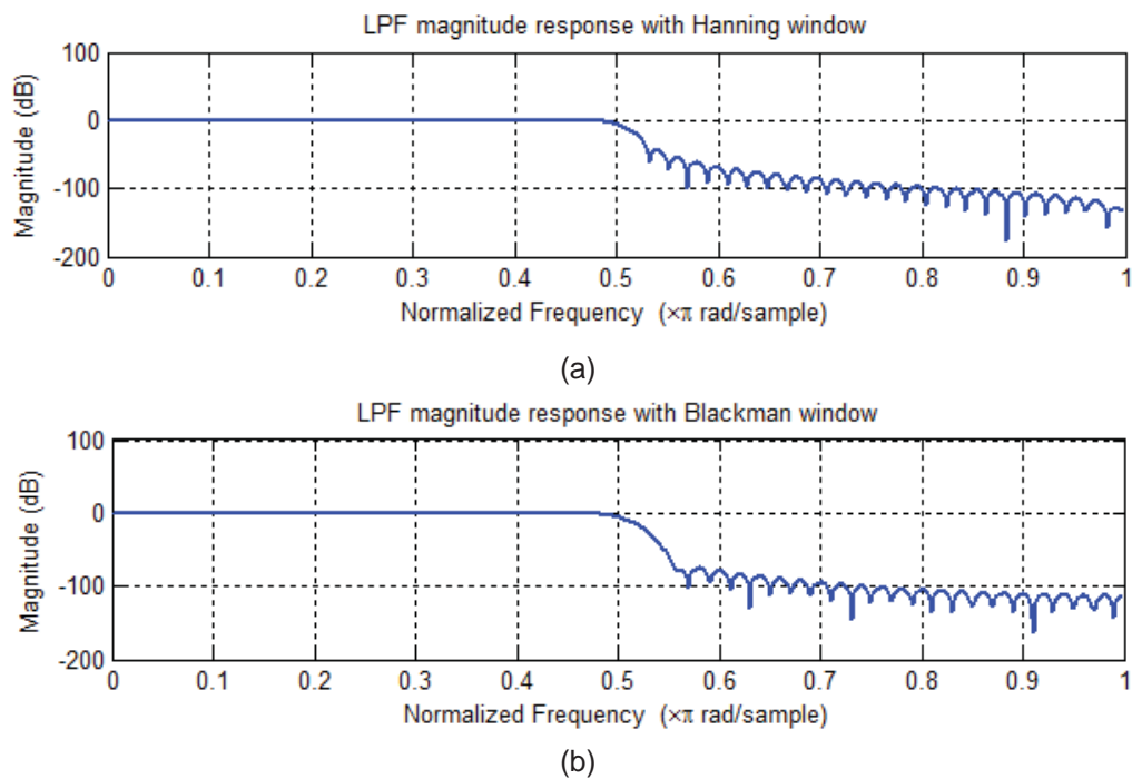
Figure 4.23: LPF design using windows (a) Hanning (b) Blackman.
