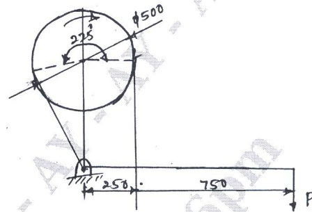
Fig.Q6(b) : All dimensions are in mm
