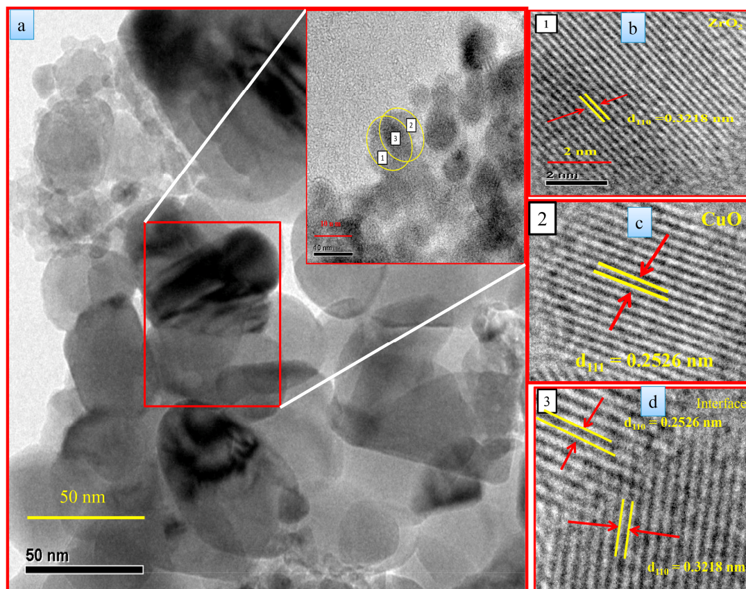
Fig. 6 (a) HRTEM image of Zr_2Cu nanocomposite (inset of (a)) The magnified region showing the interface of a typical ZrO_2 and CuO NPs, (b–d) represent the high magnification of HR-TEM images corresponding to ZrO_2 (1), CuO (2) and interface (3) region.
