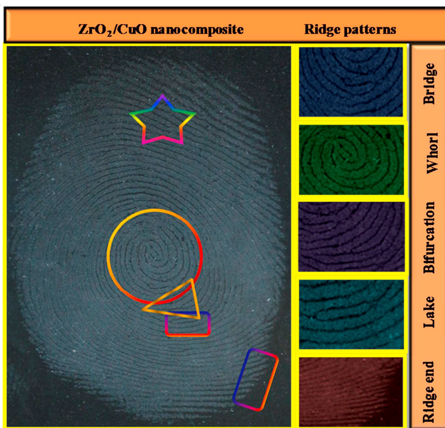
Fig. 18 Pictorial representation for enhancement of LFPs using Zr_2Cu NCO photocatalyst by dusting process & SEM image of Zr_2Cu NCO for clear observation of fingerprint ridges and particle distribution in ridges .
